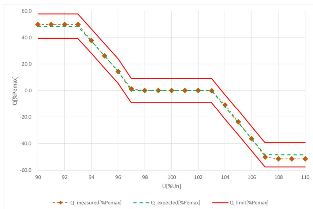
Graph of characteristic Q (U):
